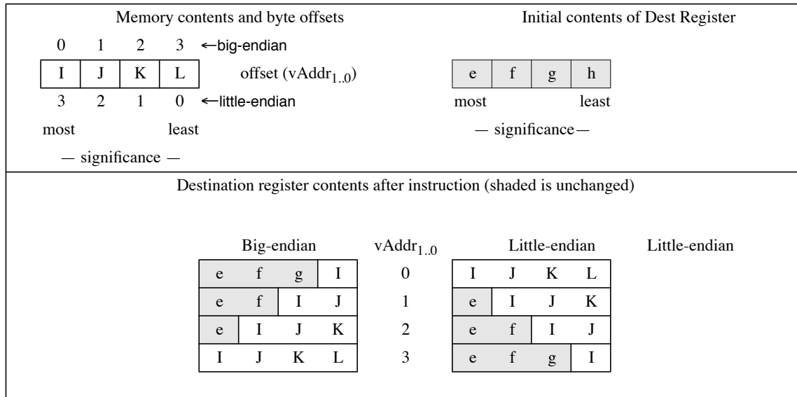
Figure 3-5 Bytes Loaded by LWL Instruction
